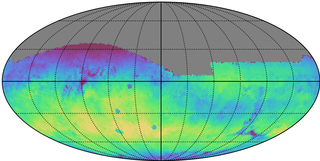
all_long_v3.4_10yrs All sky r band: Median skyBrightness
