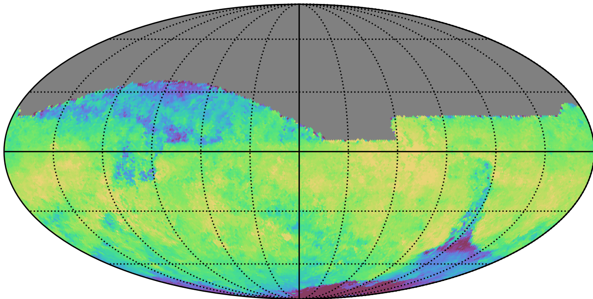
all_long_v3.4_10yrs All sky i band: Median skyBrightness
