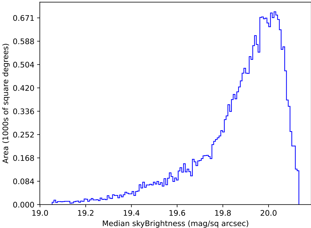
all_long_v3.4_10yrs All sky i band: Median skyBrightness
