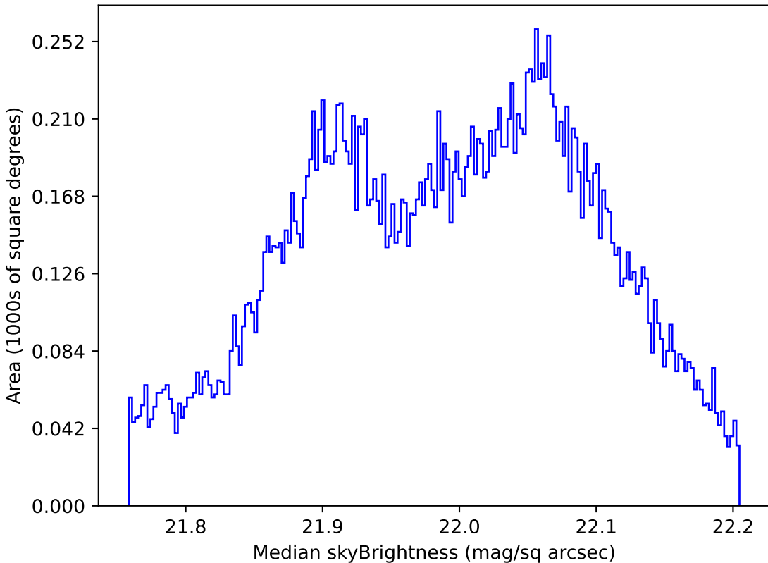
all_long_v3.4_10yrs All sky g band: Median skyBrightness
