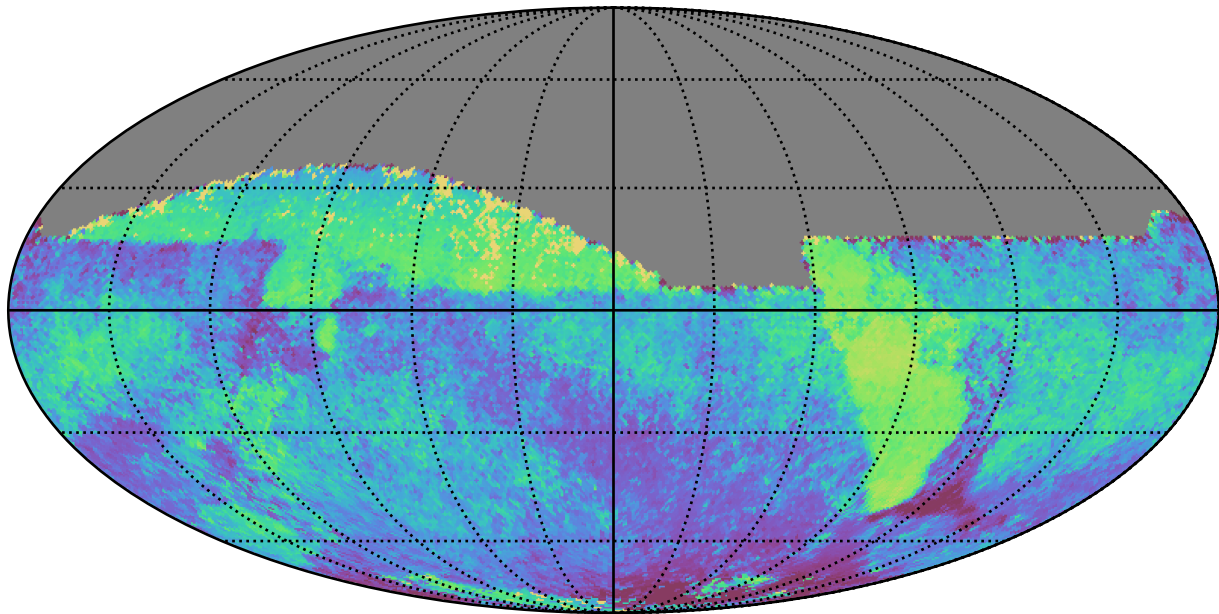
all_long_v3.4_10yrs All sky all bands: Median skyBrightness
