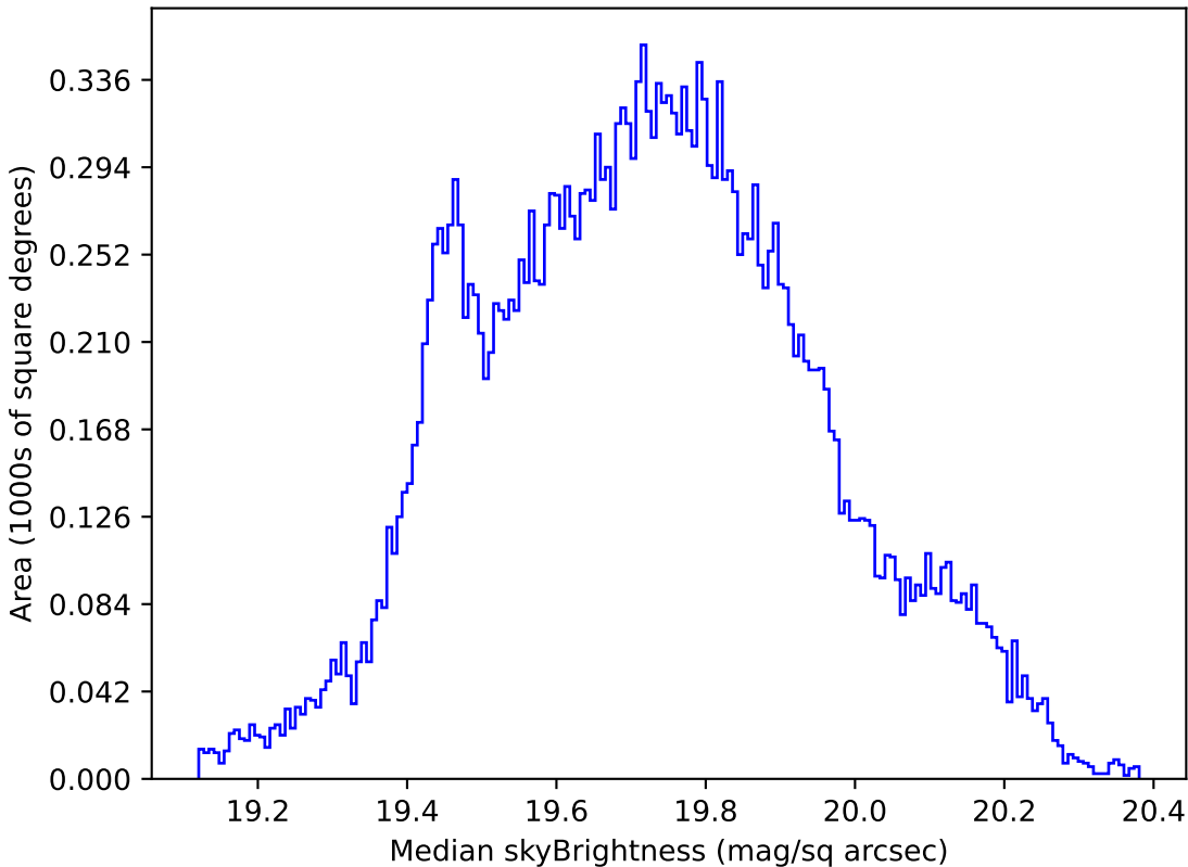
all_long_v3.4_10yrs All sky all bands: Median skyBrightness
