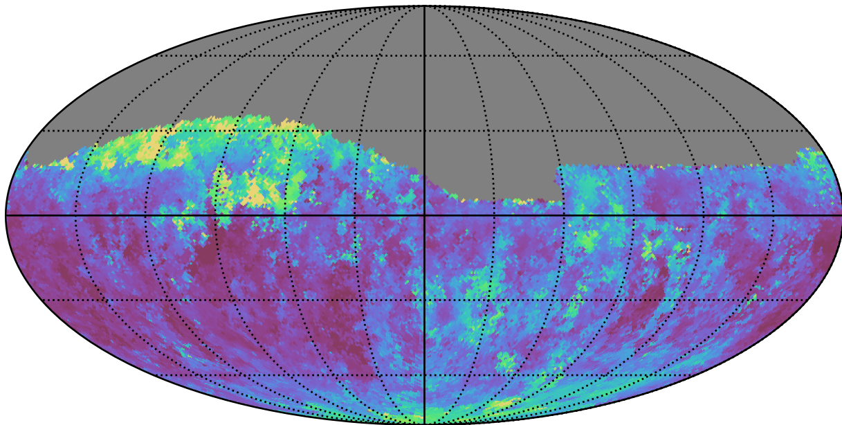
all_long_v3.4_10yrs Yr 1 z band: Median seeingGeom
