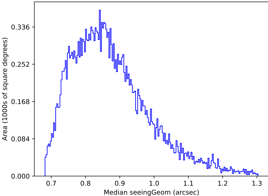
all_long_v3.4_10yrs Yr 1 z band: Median seeingGeom
