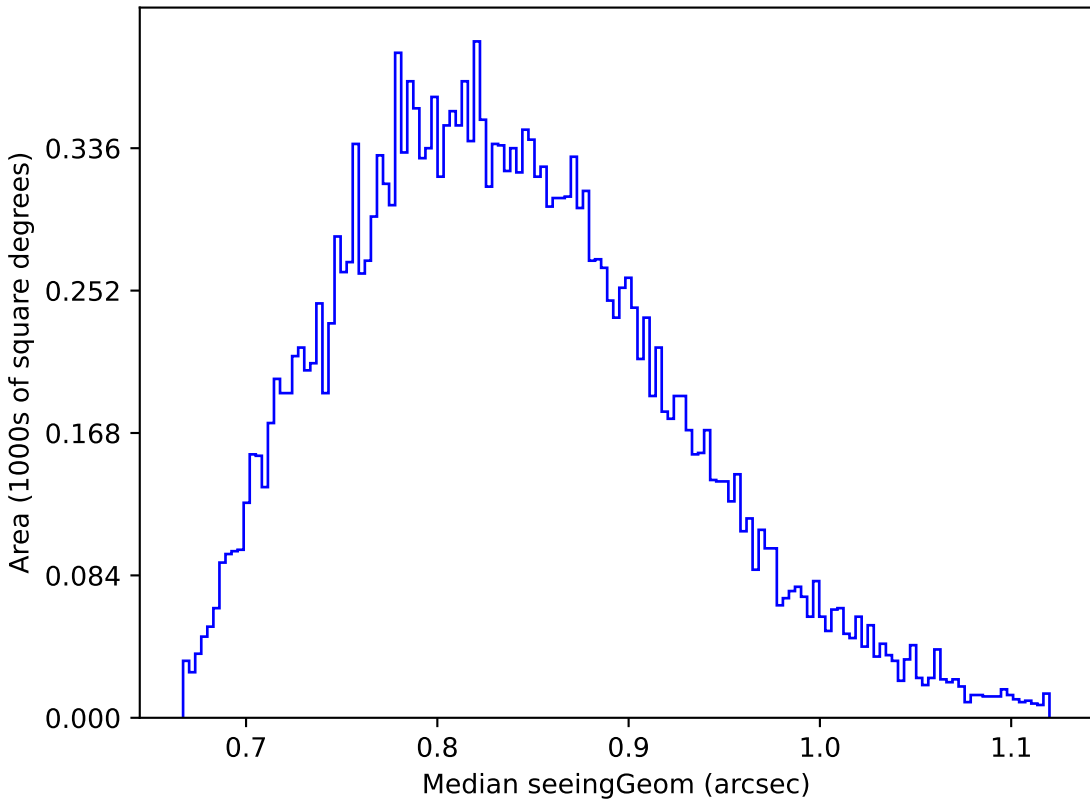
all_long_v3.4_10yrs Yr 1 y band: Median seeingGeom
