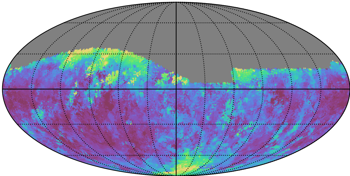
all_long_v3.4_10yrs Yr 1 r band: Median seeingGeom
