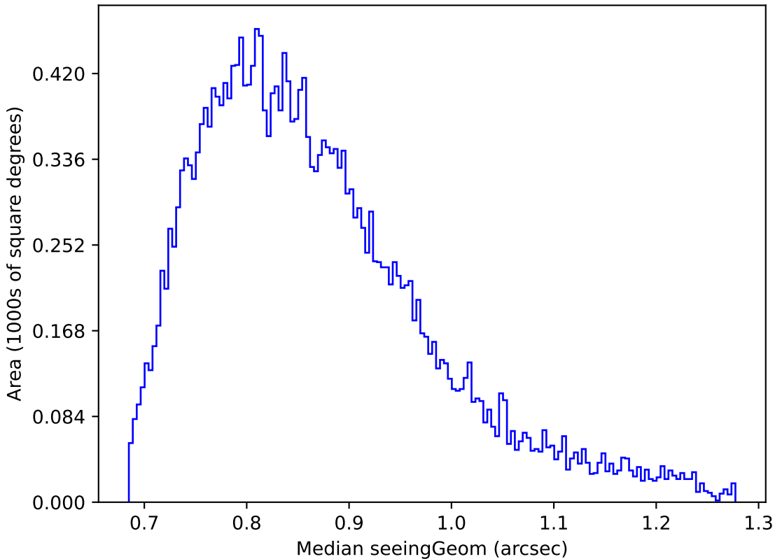
all_long_v3.4_10yrs Yr 1 r band: Median seeingGeom
