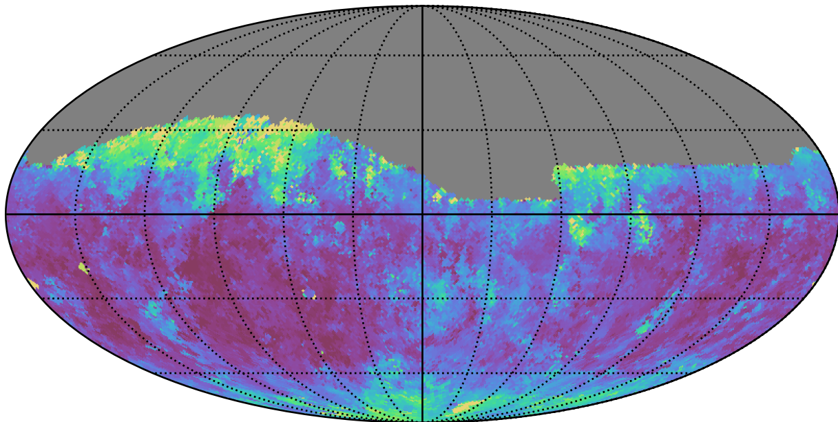
all_long_v3.4_10yrs Yr 1 i band: Median seeingGeom
