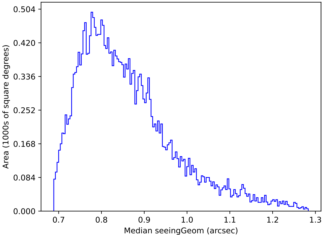
all_long_v3.4_10yrs Yr 1 i band: Median seeingGeom
