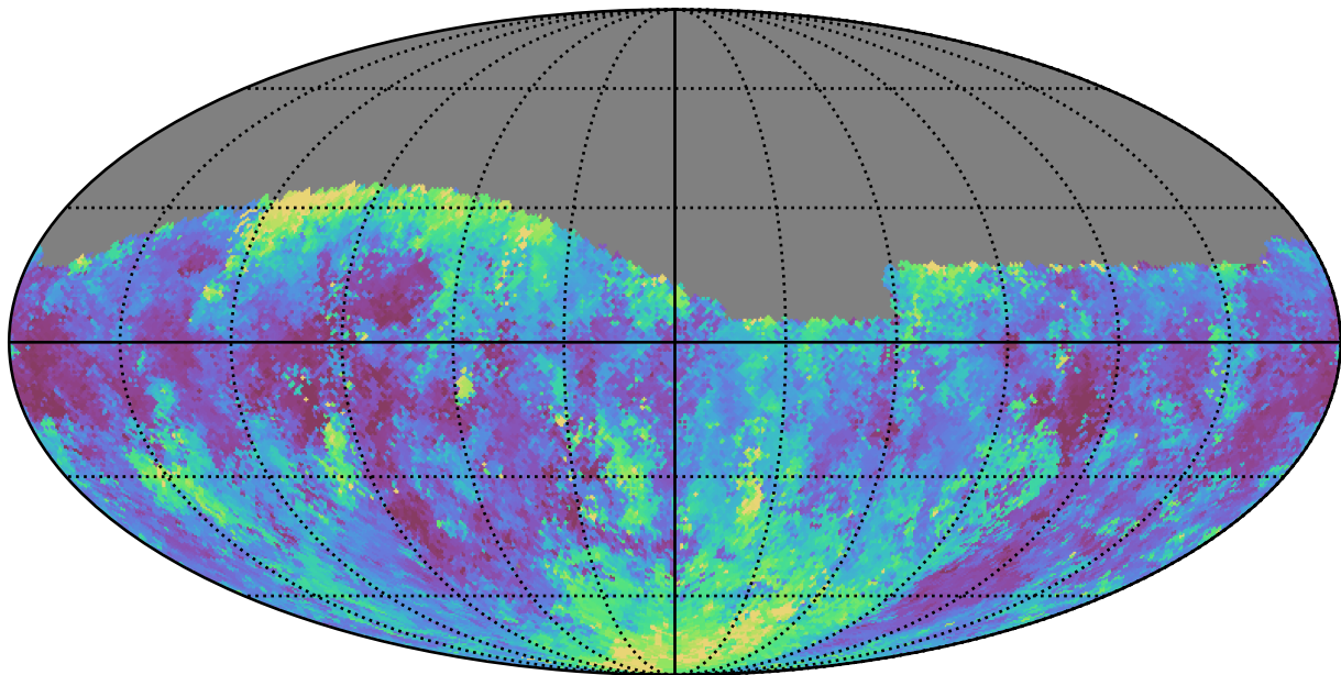
all_long_v3.4_10yrs Yr 1 g band: Median seeingGeom
