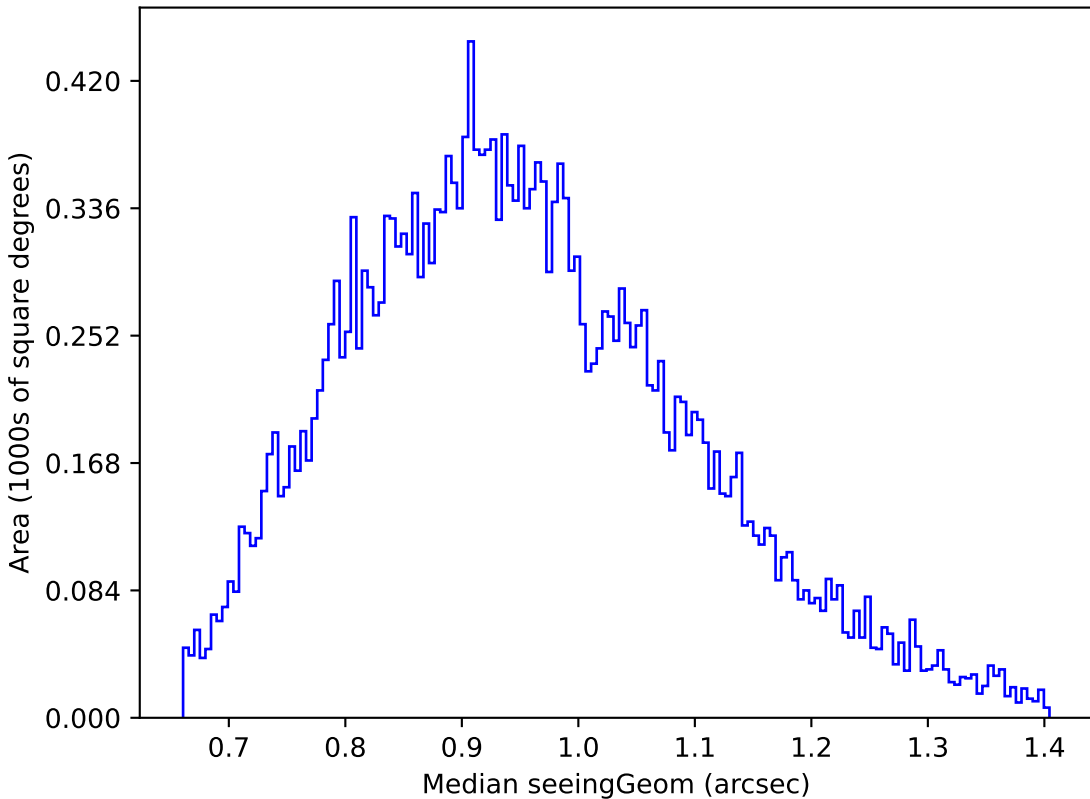
all_long_v3.4_10yrs Yr 1 g band: Median seeingGeom
