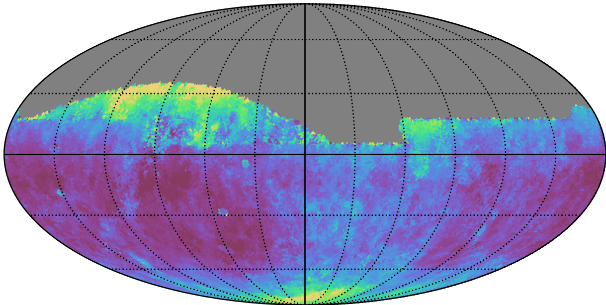
all_long_v3.4_10yrs Yr 1 all bands: Median seeingGeom
