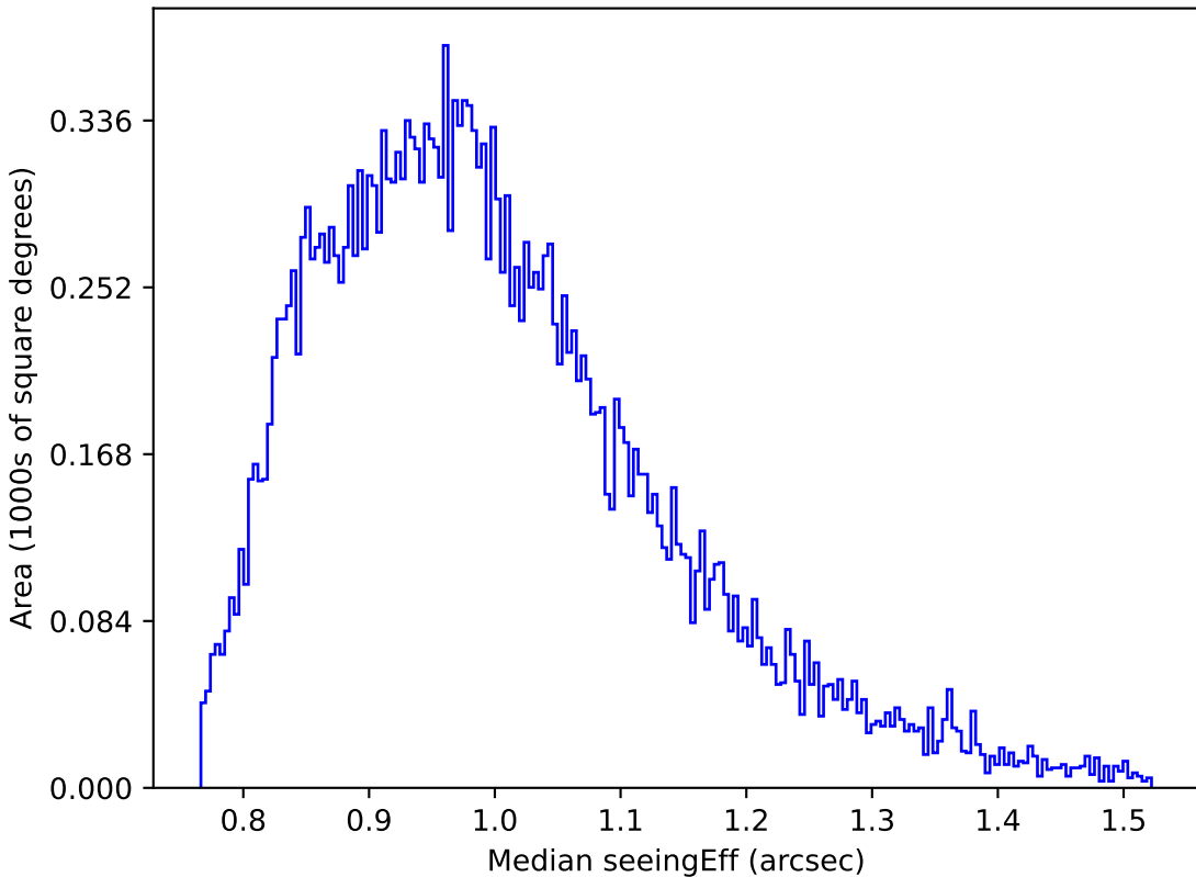
all_long_v3.4_10yrs Yr 1 z band: Median seeingEff
