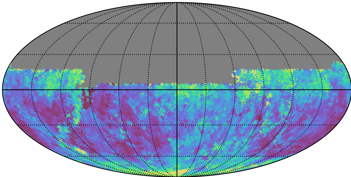
all_long_v3.4_10yrs Yr 1 y band: Median seeingEff
