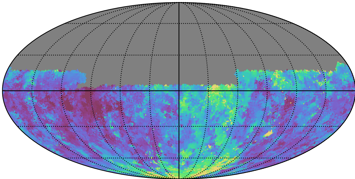
all_long_v3.4_10yrs Yr 1 u band: Median seeingEff
