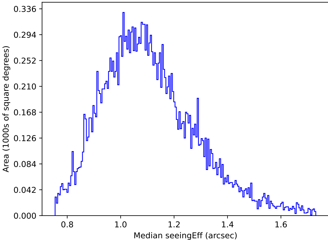
all_long_v3.4_10yrs Yr 1 u band: Median seeingEff
