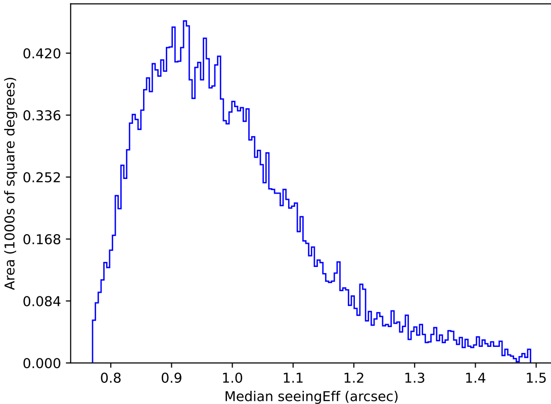
all_long_v3.4_10yrs Yr 1 r band: Median seeingEff
