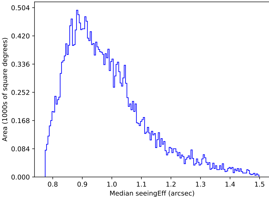
all_long_v3.4_10yrs Yr 1 i band: Median seeingEff
