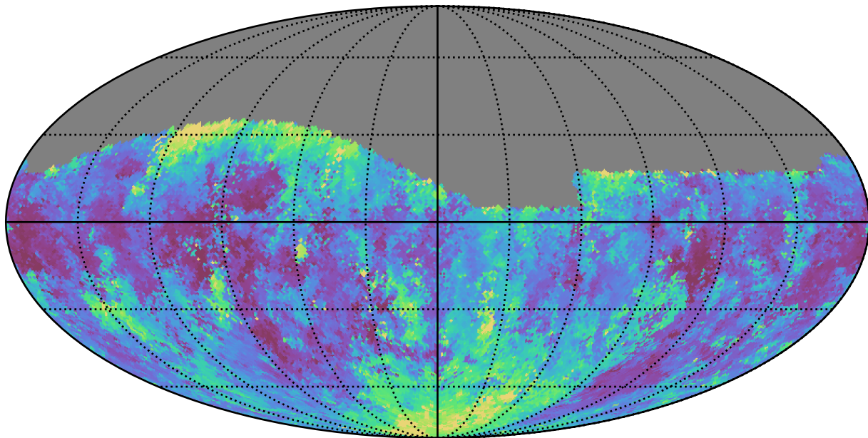
all_long_v3.4_10yrs Yr 1 g band: Median seeingEff
