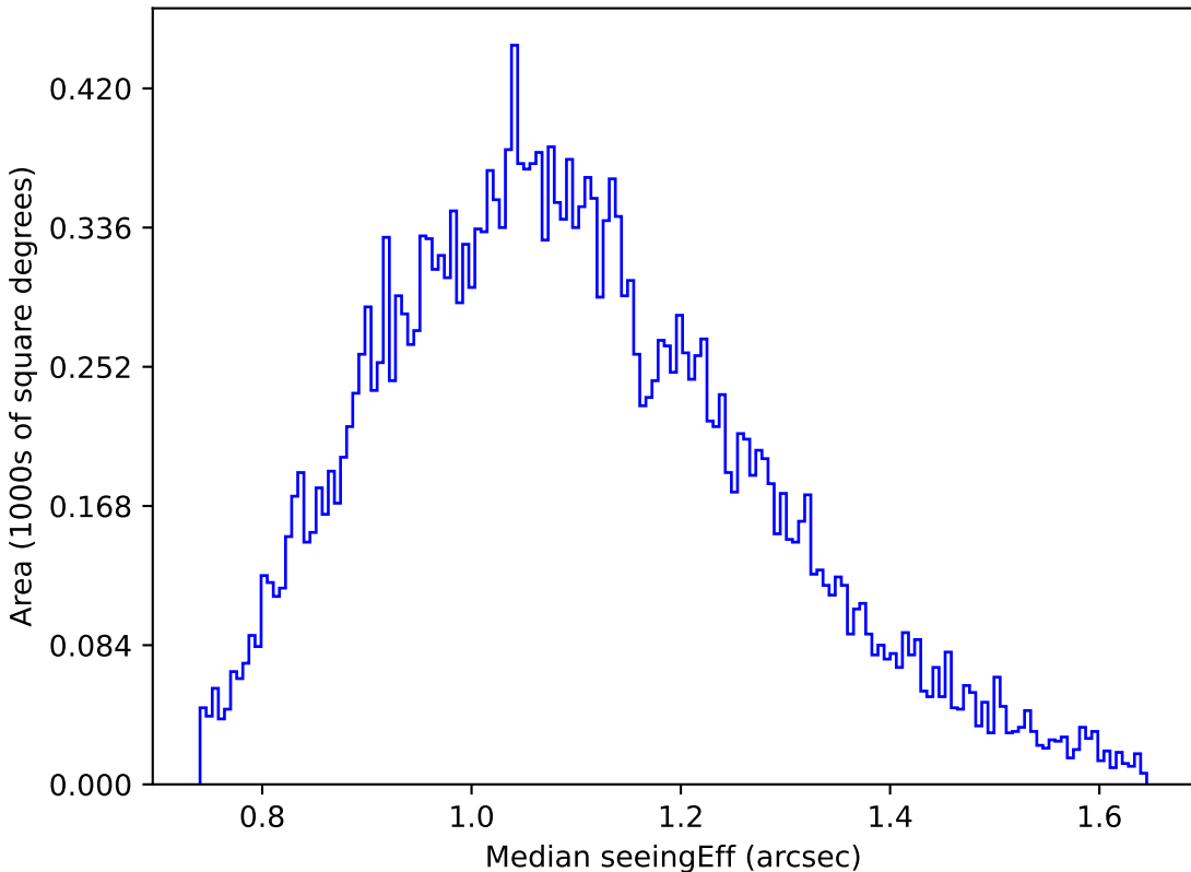
all_long_v3.4_10yrs Yr 1 g band: Median seeingEff
