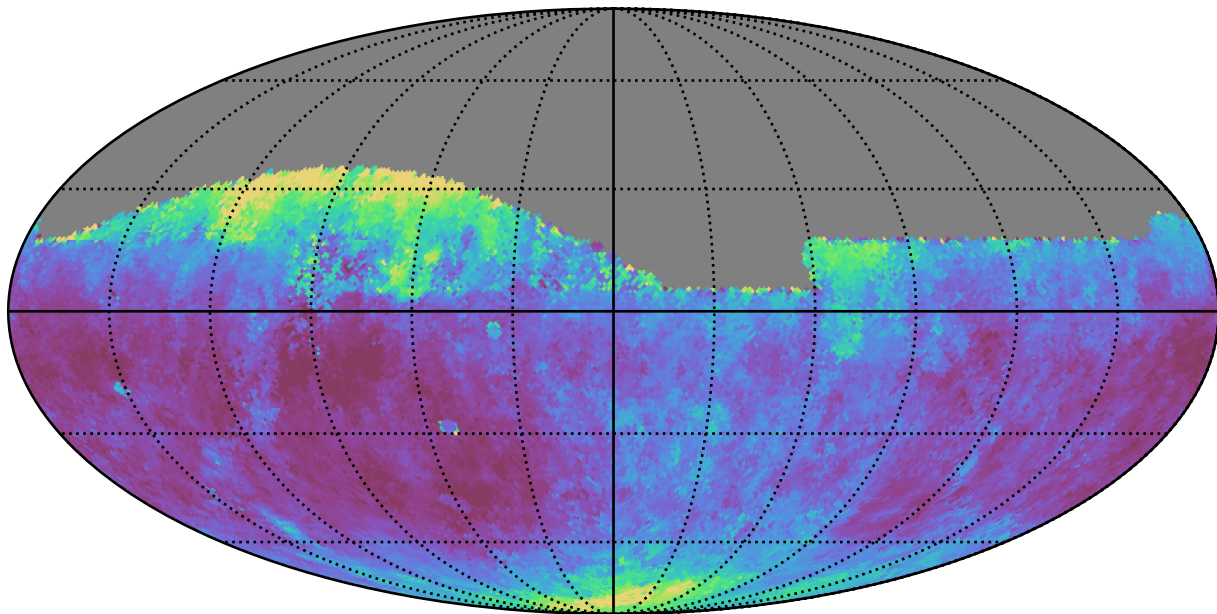
all_long_v3.4_10yrs Yr 1 all bands: Median seeingEff
