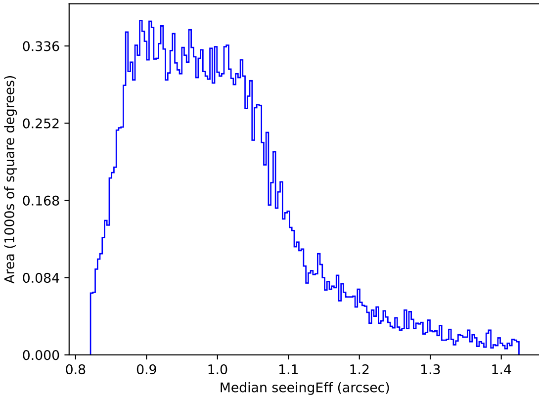
all_long_v3.4_10yrs Yr 1 all bands: Median seeingEff
