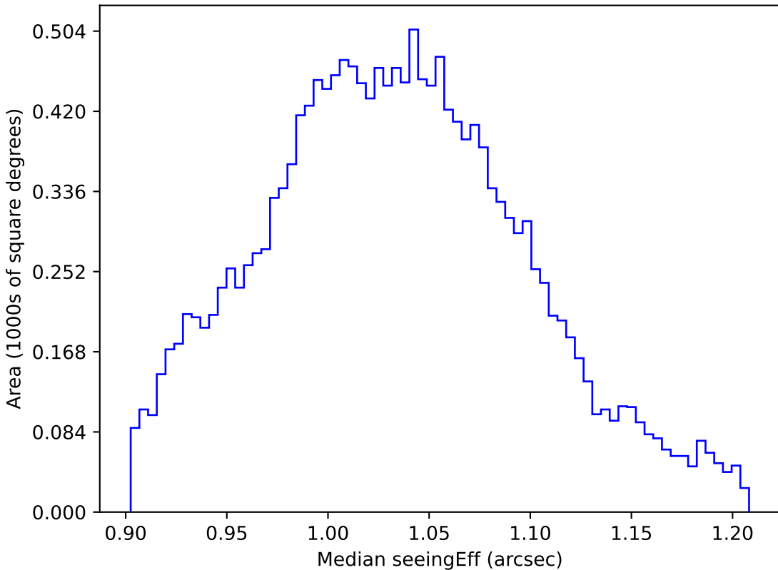
all_long_v3.4_10yrs WFD z band: Median seeingEff
