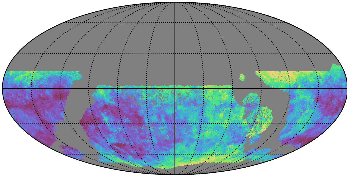
all_long_v3.4_10yrs WFD u band: Median seeingEff
