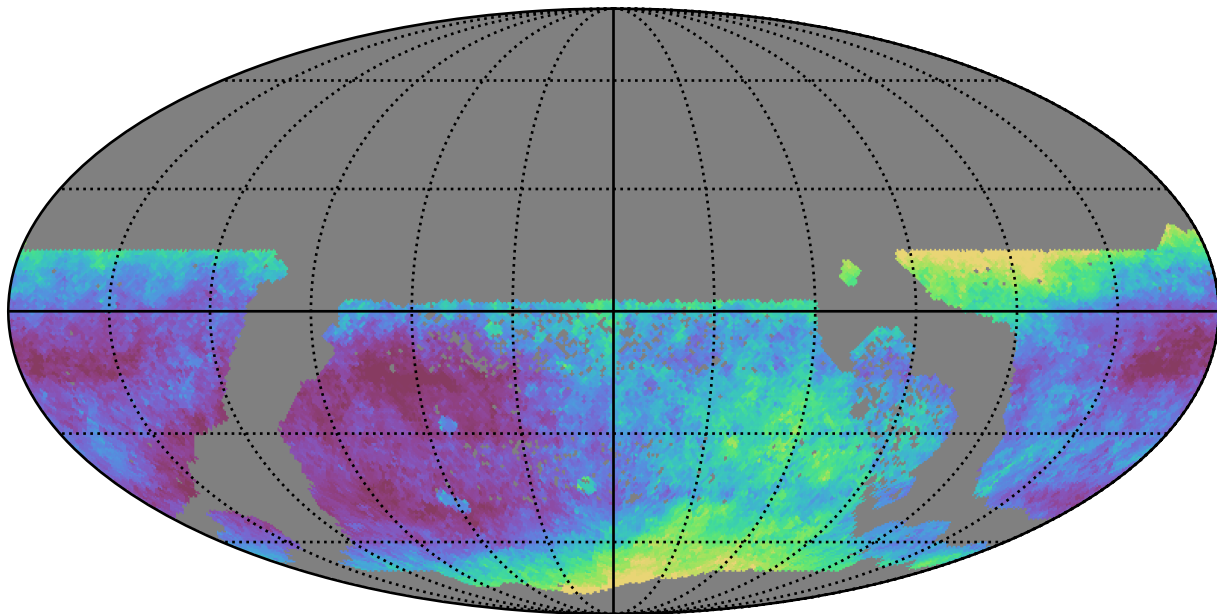
all_long_v3.4_10yrs WFD r band: Median seeingEff
