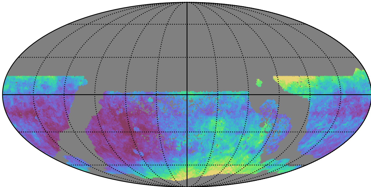
all_long_v3.4_10yrs WFD i band: Median seeingEff
