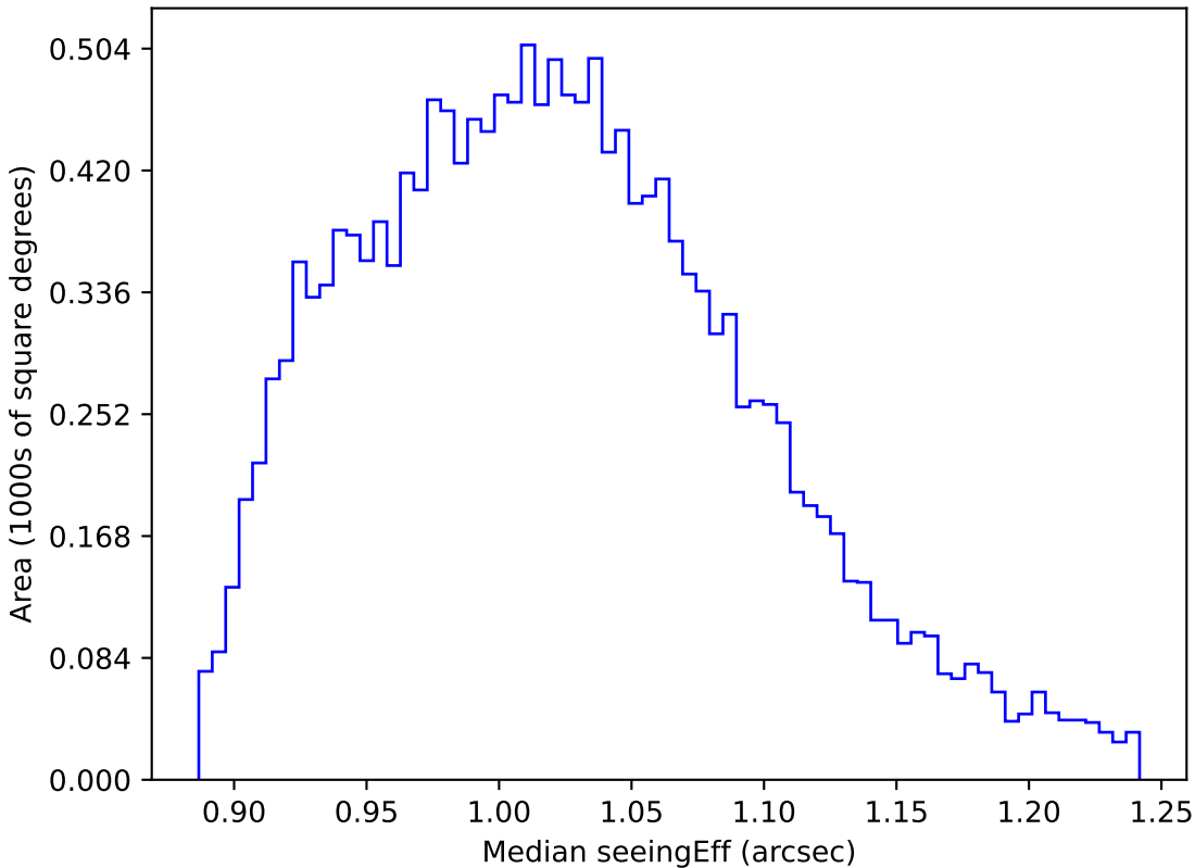
all_long_v3.4_10yrs WFD i band: Median seeingEff
