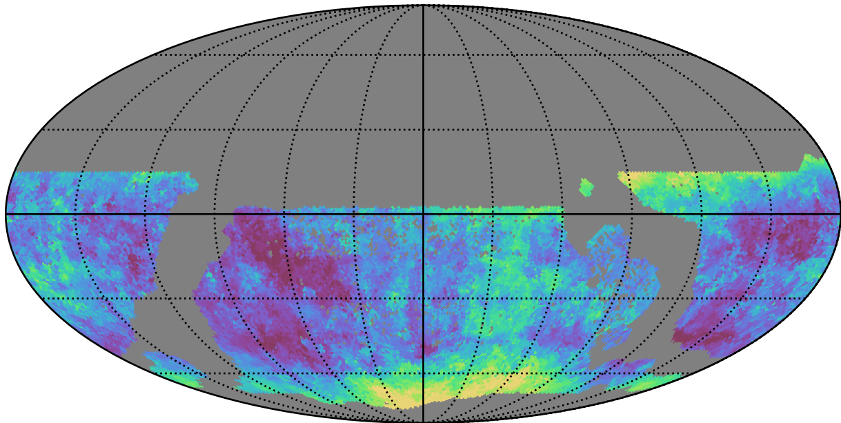
all_long_v3.4_10yrs WFD g band: Median seeingEff
