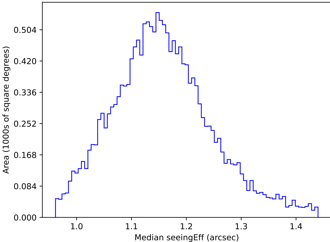
all_long_v3.4_10yrs WFD g band: Median seeingEff
