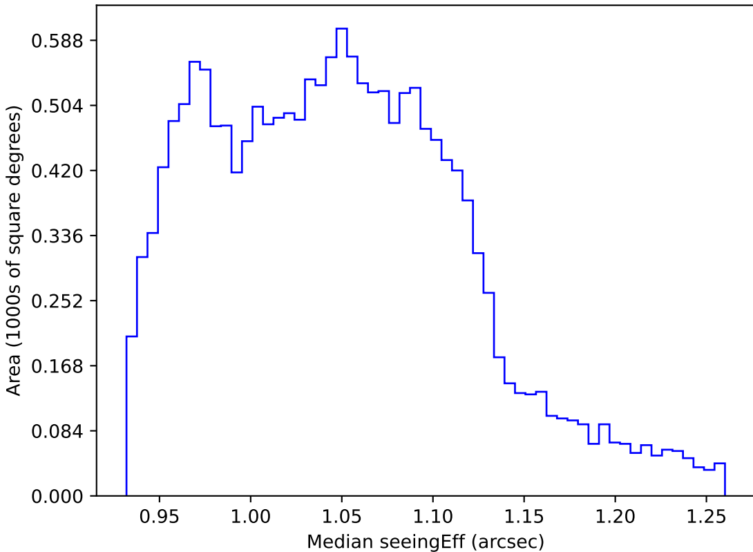
all_long_v3.4_10yrs WFD all bands: Median seeingEff
