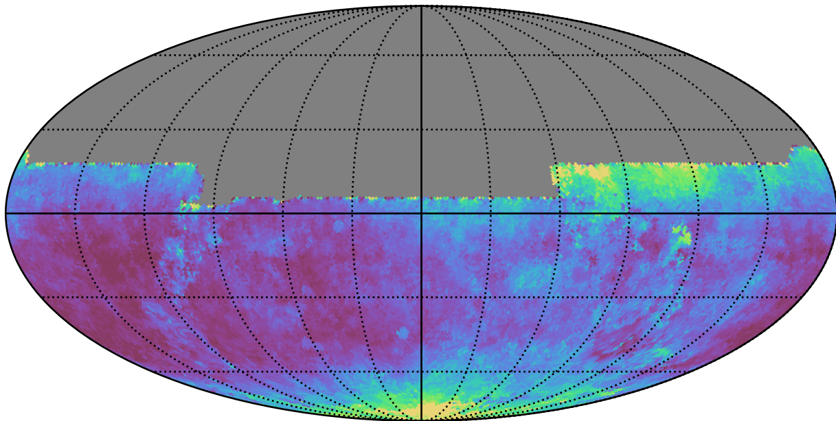
all_long_v3.4_10yrs All sky y band: Median seeingEff
