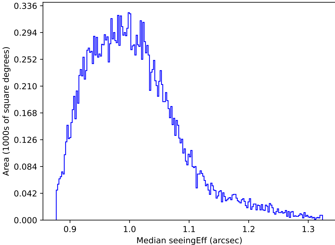
all_long_v3.4_10yrs All sky y band: Median seeingEff
