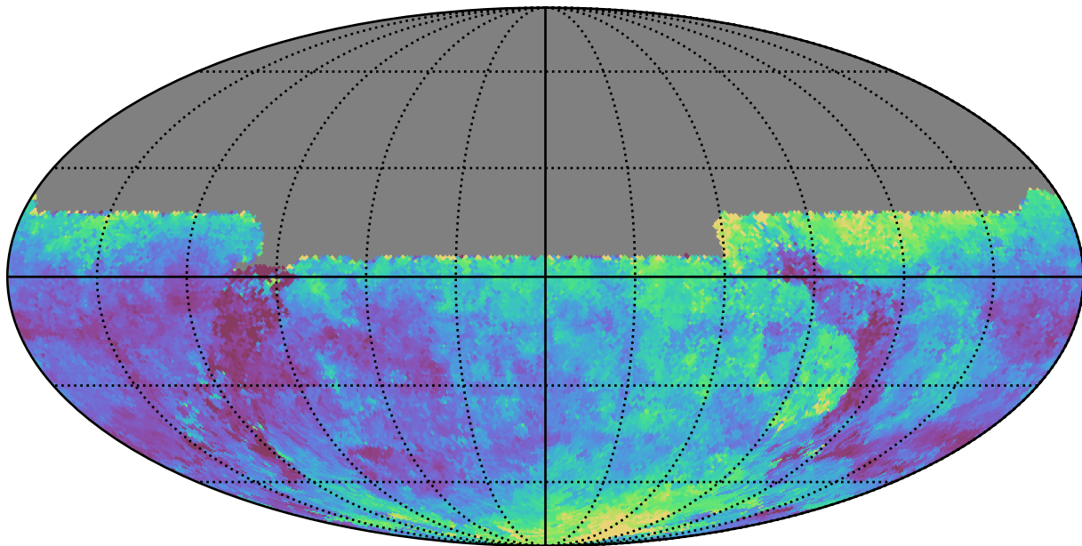
all_long_v3.4_10yrs All sky u band: Median seeingEff
