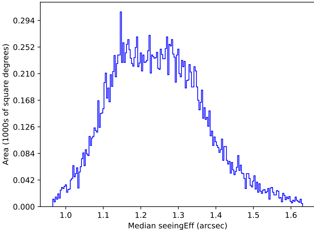
all_long_v3.4_10yrs All sky u band: Median seeingEff
