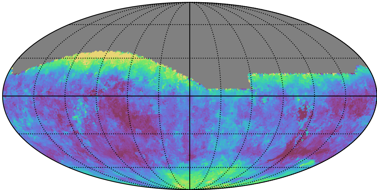
all_long_v3.4_10yrs All sky g band: Median seeingEff
