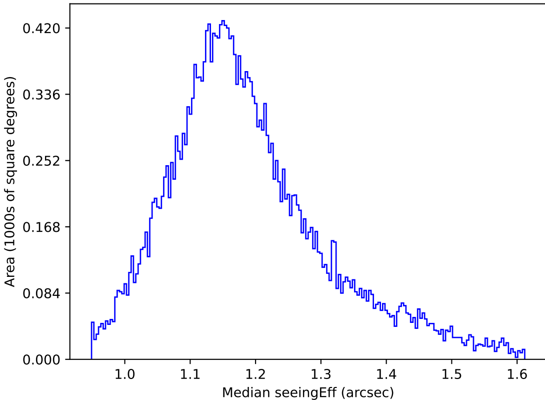
all_long_v3.4_10yrs All sky g band: Median seeingEff
