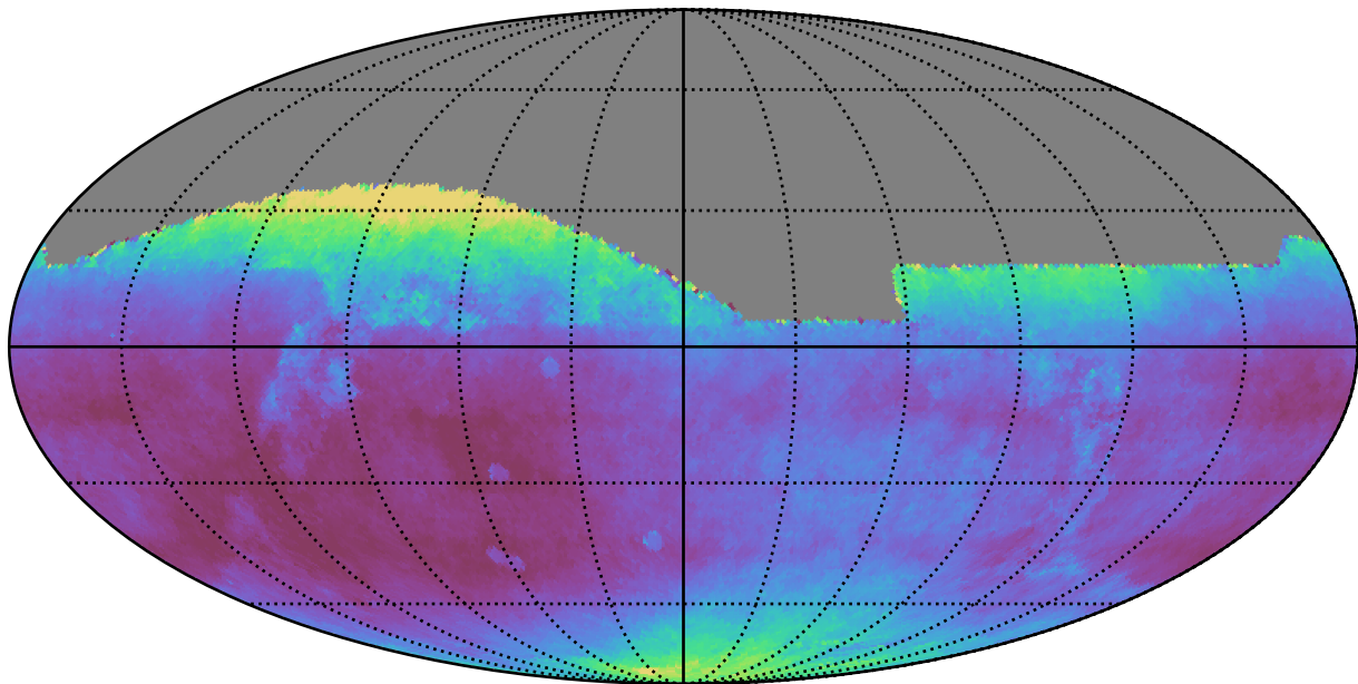
all_long_v3.4_10yrs All sky all bands: Median seeingEff
