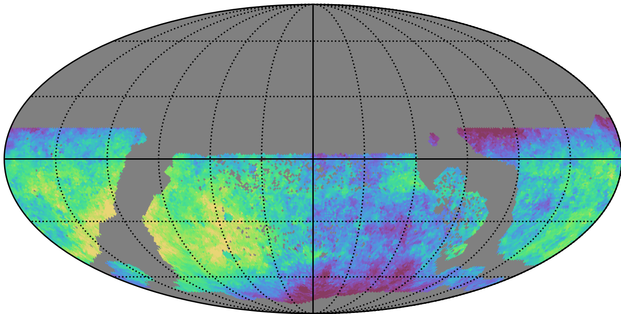
all_long_v3.4_10yrs WFD z band: Median saturation_mag
