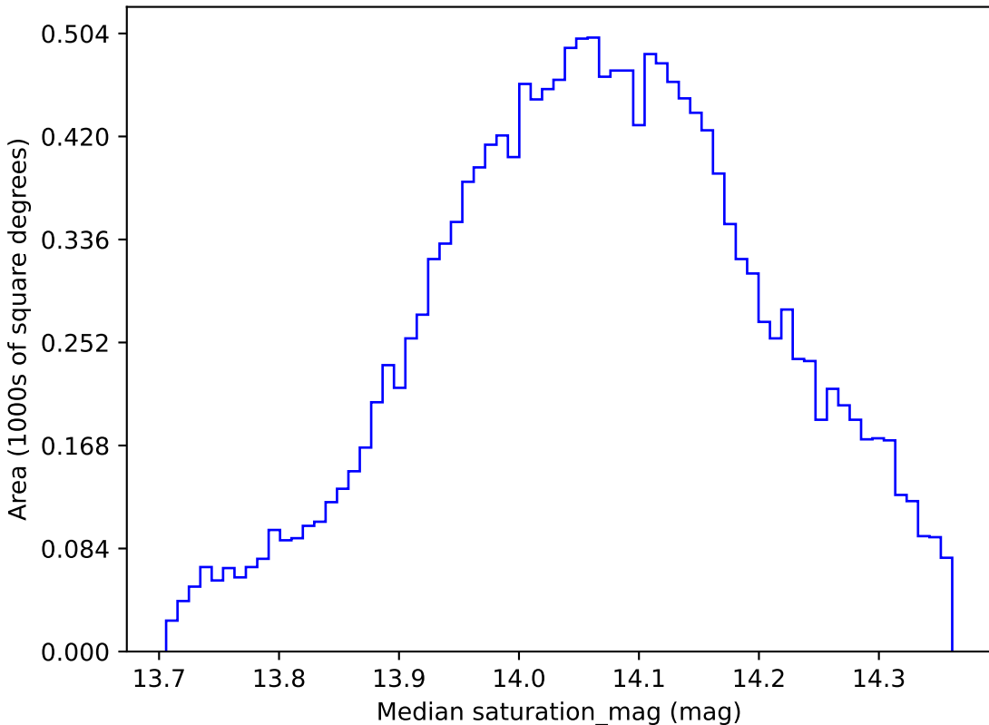
all_long_v3.4_10yrs WFD z band: Median saturation_mag
