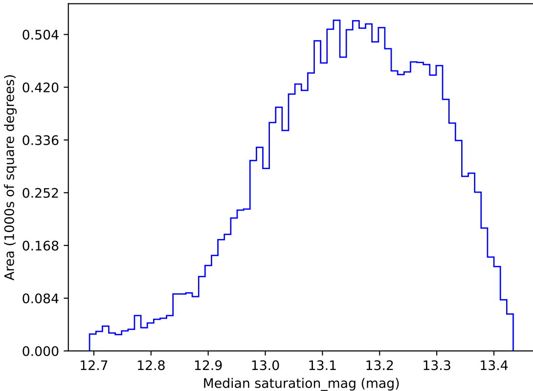
all_long_v3.4_10yrs WFD y band: Median saturation_mag
