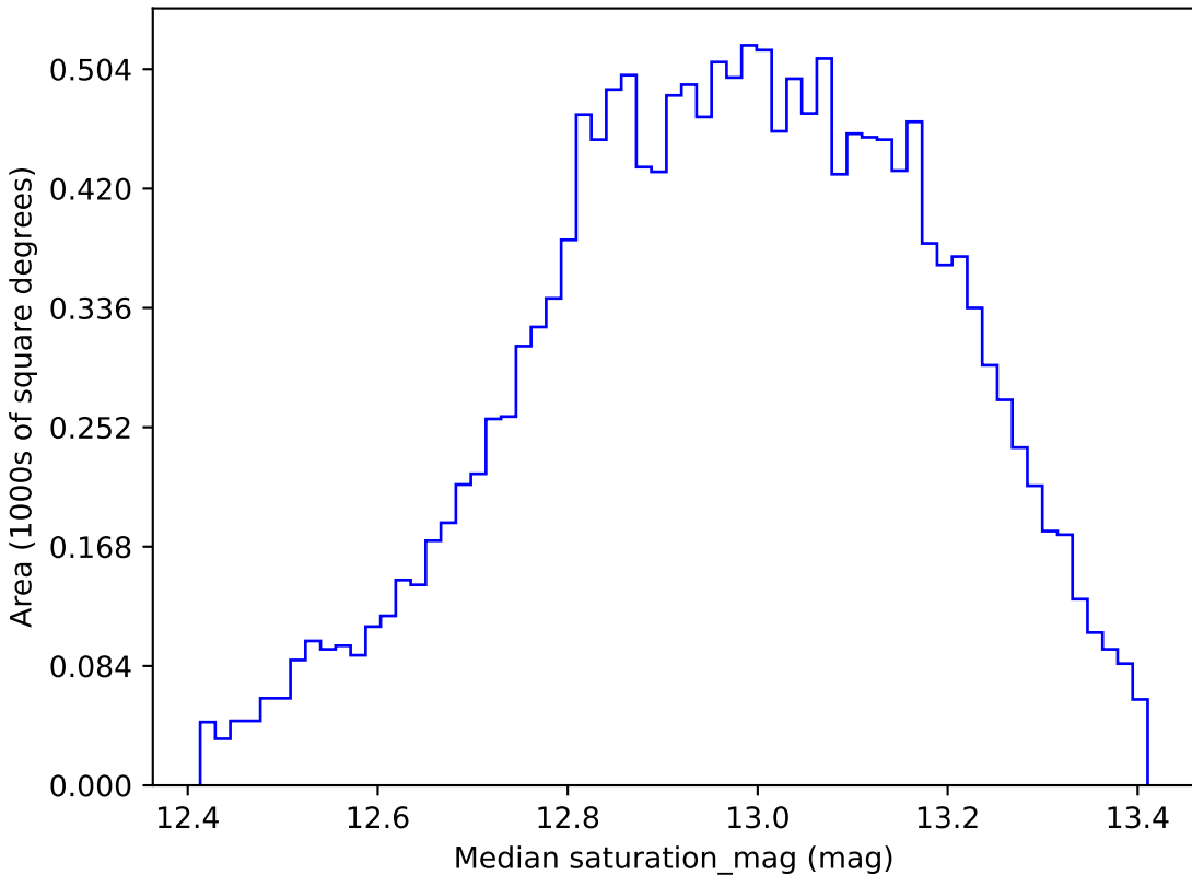
all_long_v3.4_10yrs WFD u band: Median saturation_mag
