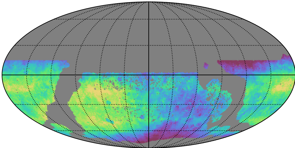
all_long_v3.4_10yrs WFD r band: Median saturation_mag
