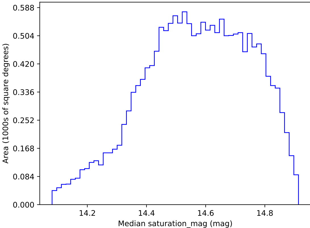
all_long_v3.4_10yrs WFD r band: Median saturation_mag
