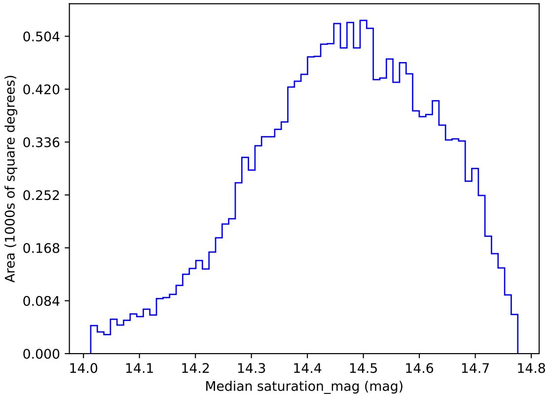
all_long_v3.4_10yrs WFD i band: Median saturation_mag
