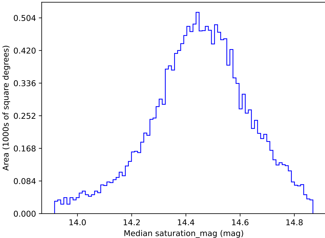
all_long_v3.4_10yrs WFD g band: Median saturation_mag
