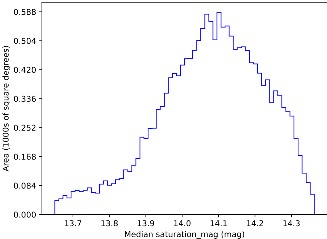
all_long_v3.4_10yrs WFD all bands: Median saturation_mag
